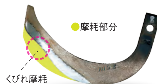
くびれ摩耗
